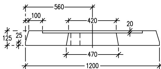
SECTIONAL ELEVATION A-A
