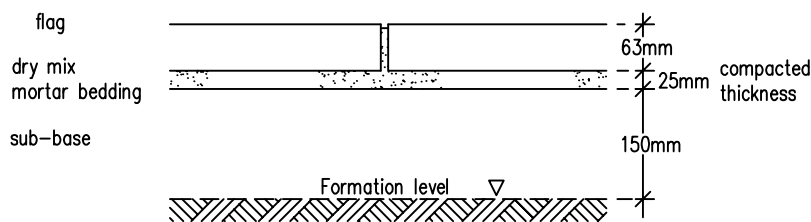
SECTIONAL ELEVATION
